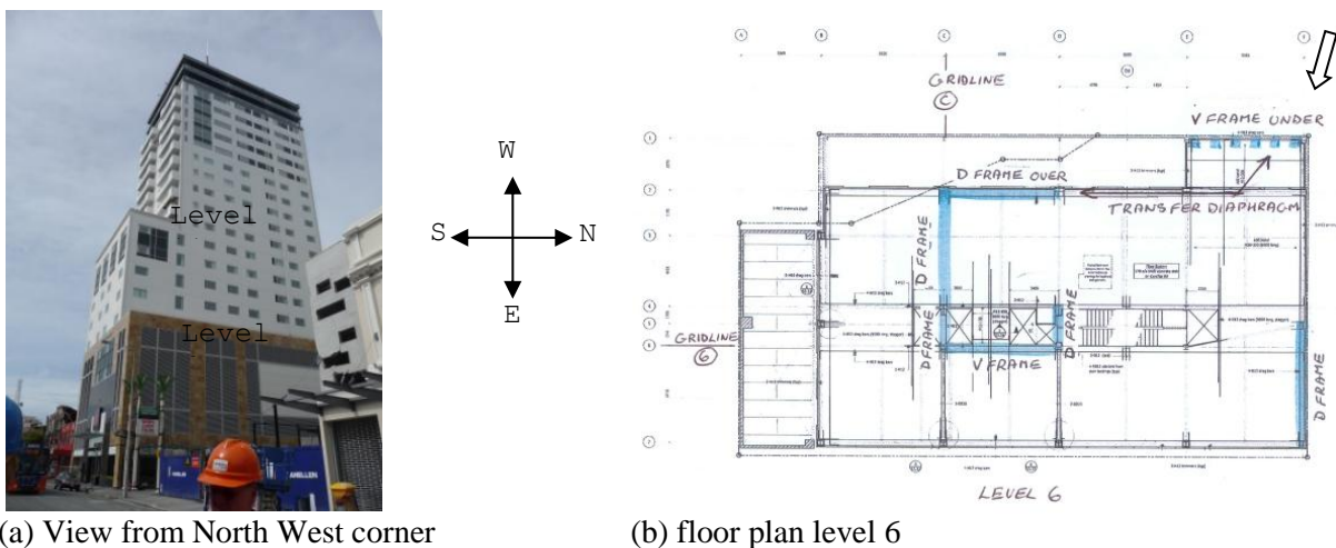
Figure 6 Pacific Tower [Photo by C Clifton, Floor Plans from S Gardiner] (the arrows in (b) show the direction of the view in (a))
