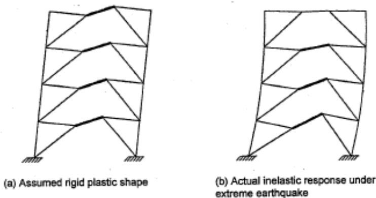
Figure 5 EBF plastic collapse mechanisms
