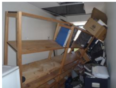
(b) Collapsed ceilings and contents [G Banks]
