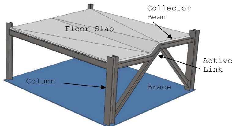
Figure 3 Floor slab contribution to EBF strength and stiffness
